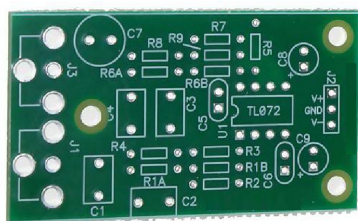
PCB
