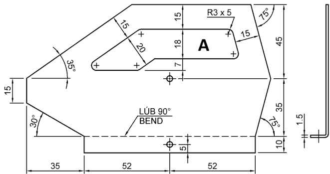
Side panel
