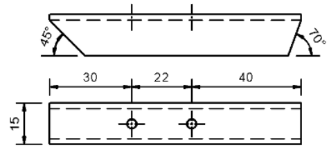
Centre Support
