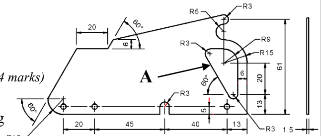
Side Panel
