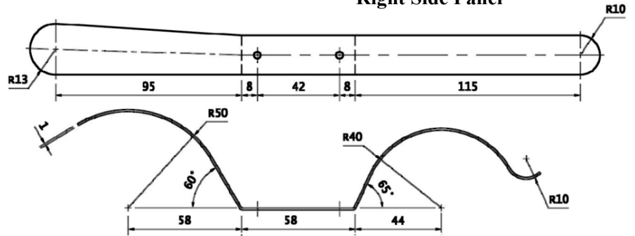
Right Mudguard
