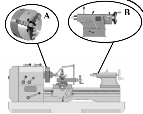
Centre Lathe
