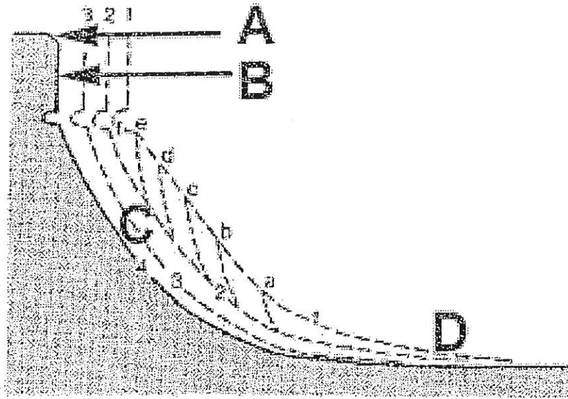
Figure 2.3 : Slope Elements
