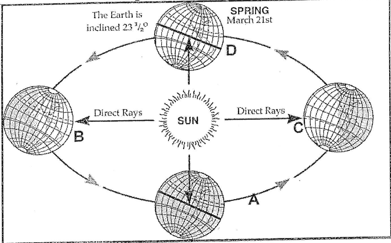
Figure 1.3 : Earth Movements
