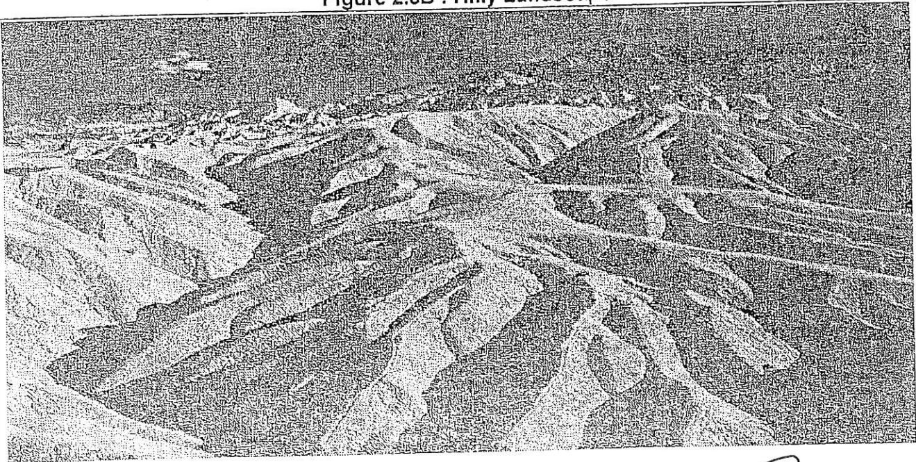
Figure 2.8B : Hilly Landscape
